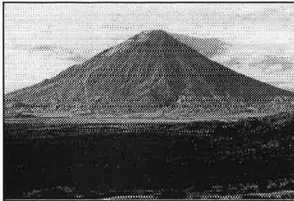
Volcan Ol Doinyo Lengai, Tanzanie
